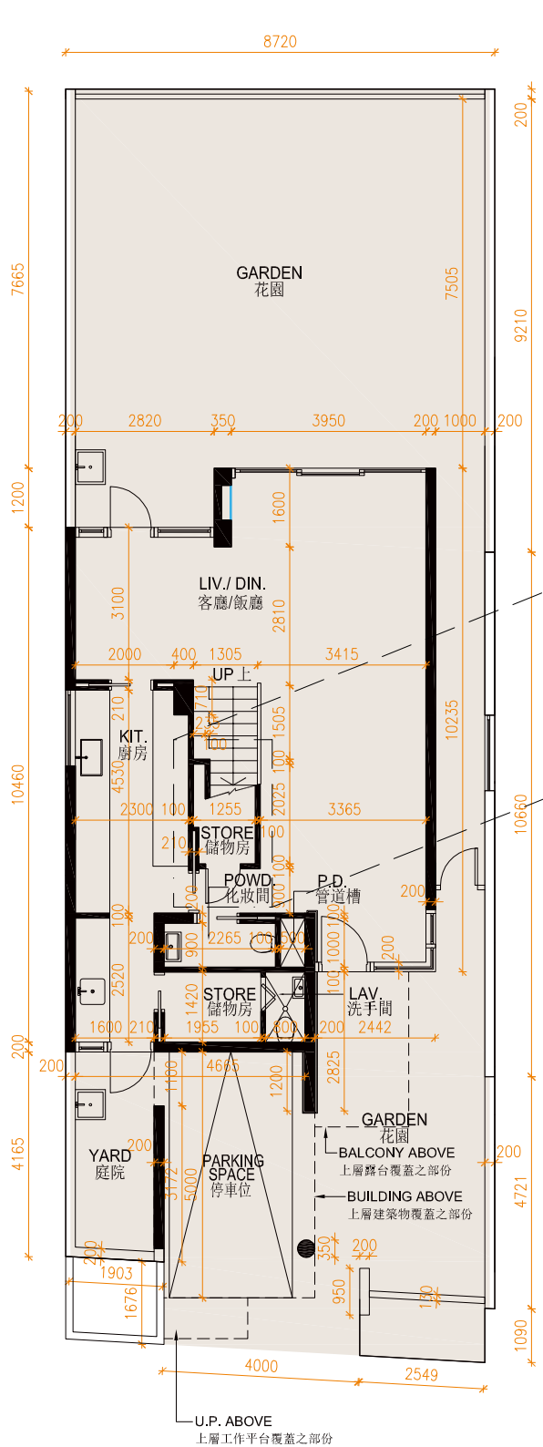
AS-BUILT PART PLAN OF FIRST FLOOR 一樓實際建造部份平面圖
