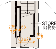
AS-BUILT PART PLAN OF GROUND FLOOR 地下實際建造部份平面圖
