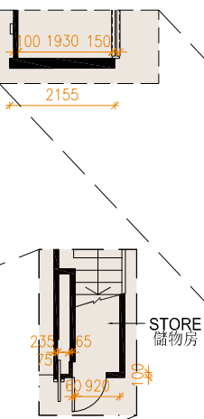
AS-BUILT PART PLAN OF GROUND FLOOR 地下實際建造部份平面圖
