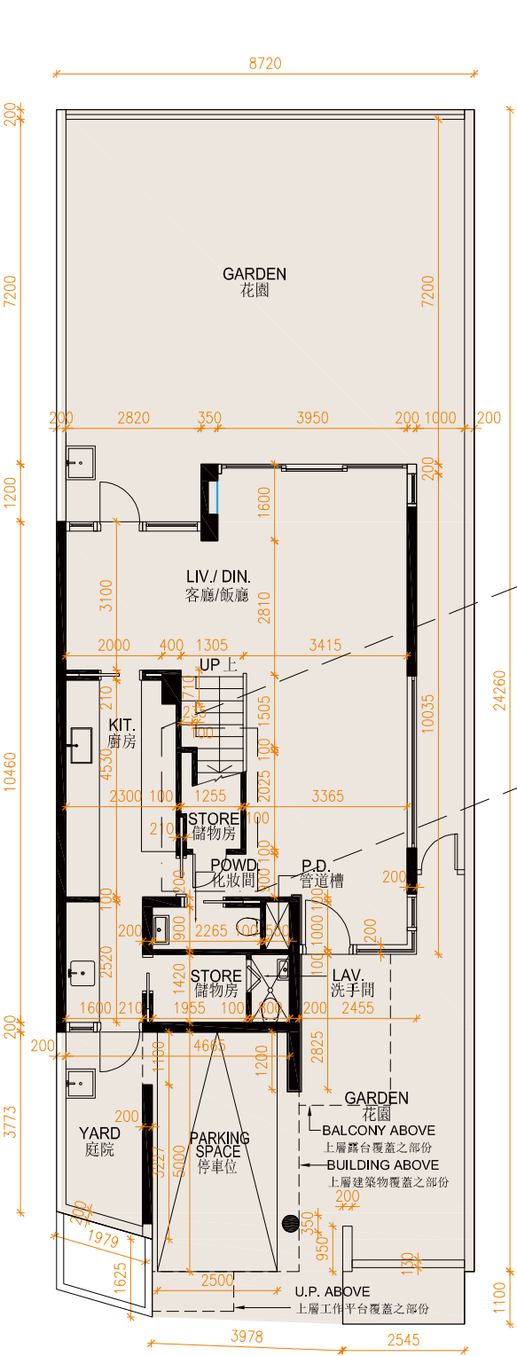
AS-BUILT PART PLAN OF FIRST FLOOR 一樓實際建造部份平面圖
