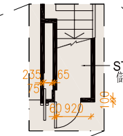
AS-BUILT PART PLAN OF GROUND FLOOR 地下實際建造部份平面圖
