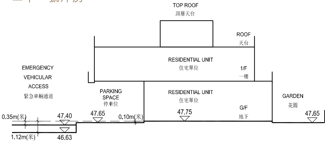
CROSS-SECTION PLAN 21-21 橫截面圖 21-21
