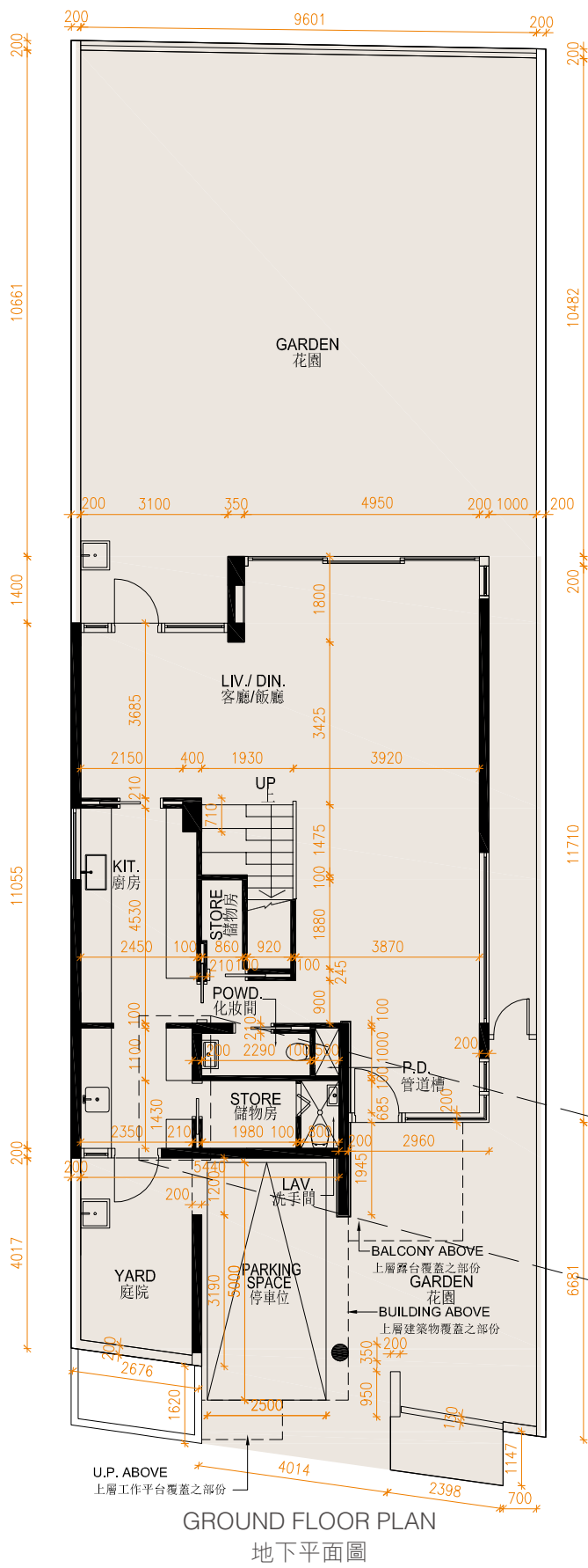
AS-BUILT PART PLAN OF GROUND FLOOR 地下實際建造部份平面圖
